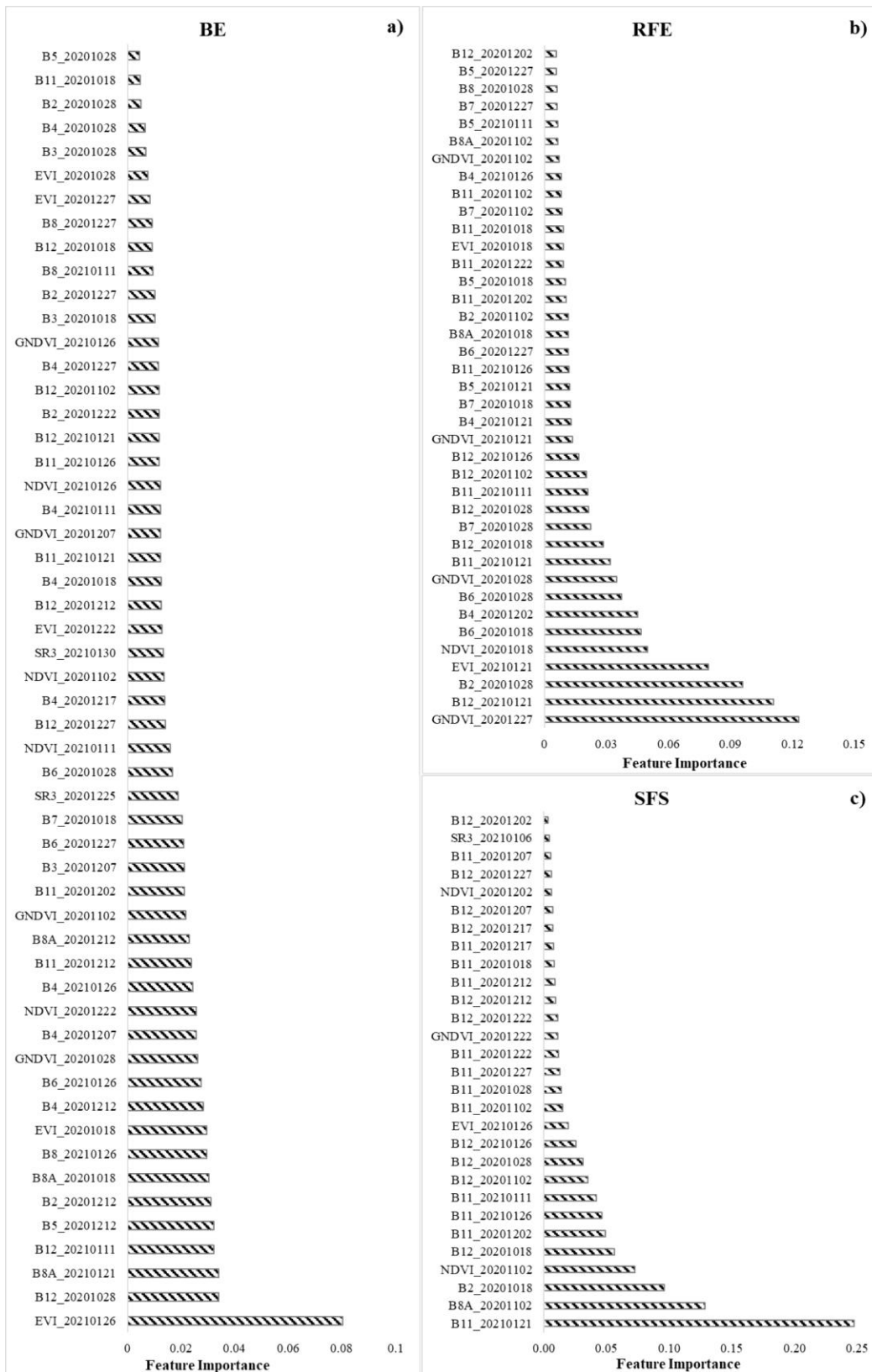
Figure 7. Feature importance for the maximum performance achieved for the dataset 4 by the 80/20 data split and XGBoost with FS technique (a) BE, (b) RFE, and (c) SFS.
