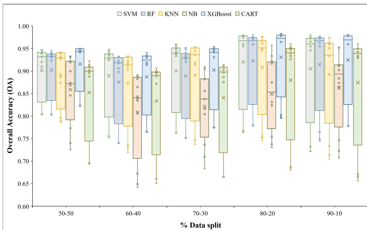
Figure 6. Box-and-whisker plot for the OA for ML classifier performance under different data split.
