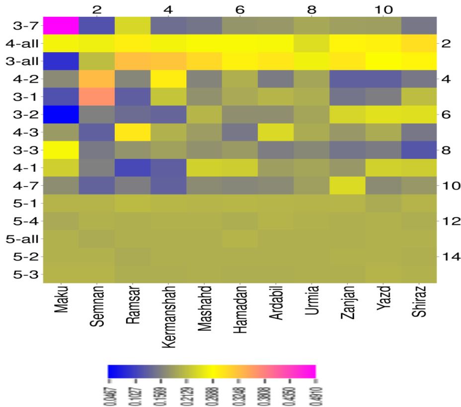
Figure 5. Heat map of weights obtained from Shannon's entropy in the monthly scale for all stations
