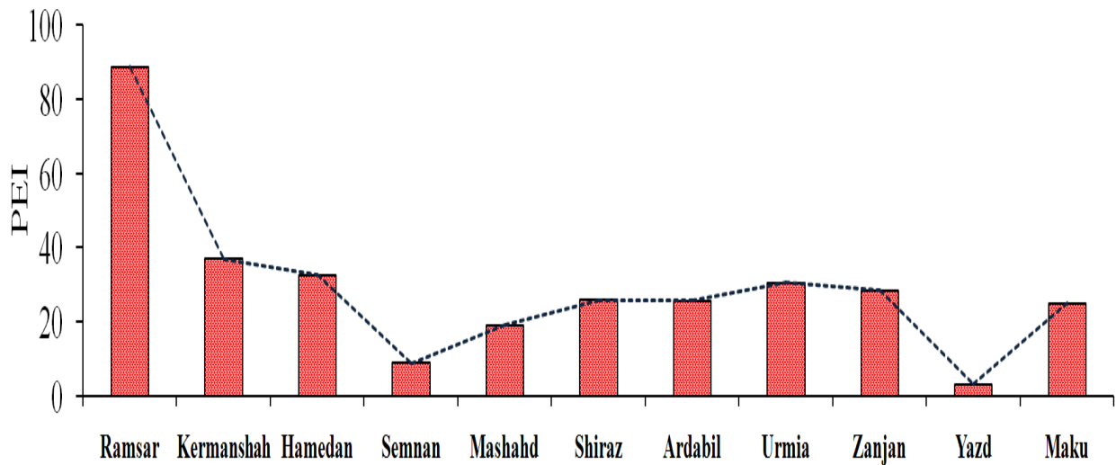
Figure 2. The climate of the studied stations with the PEI climate classification method
