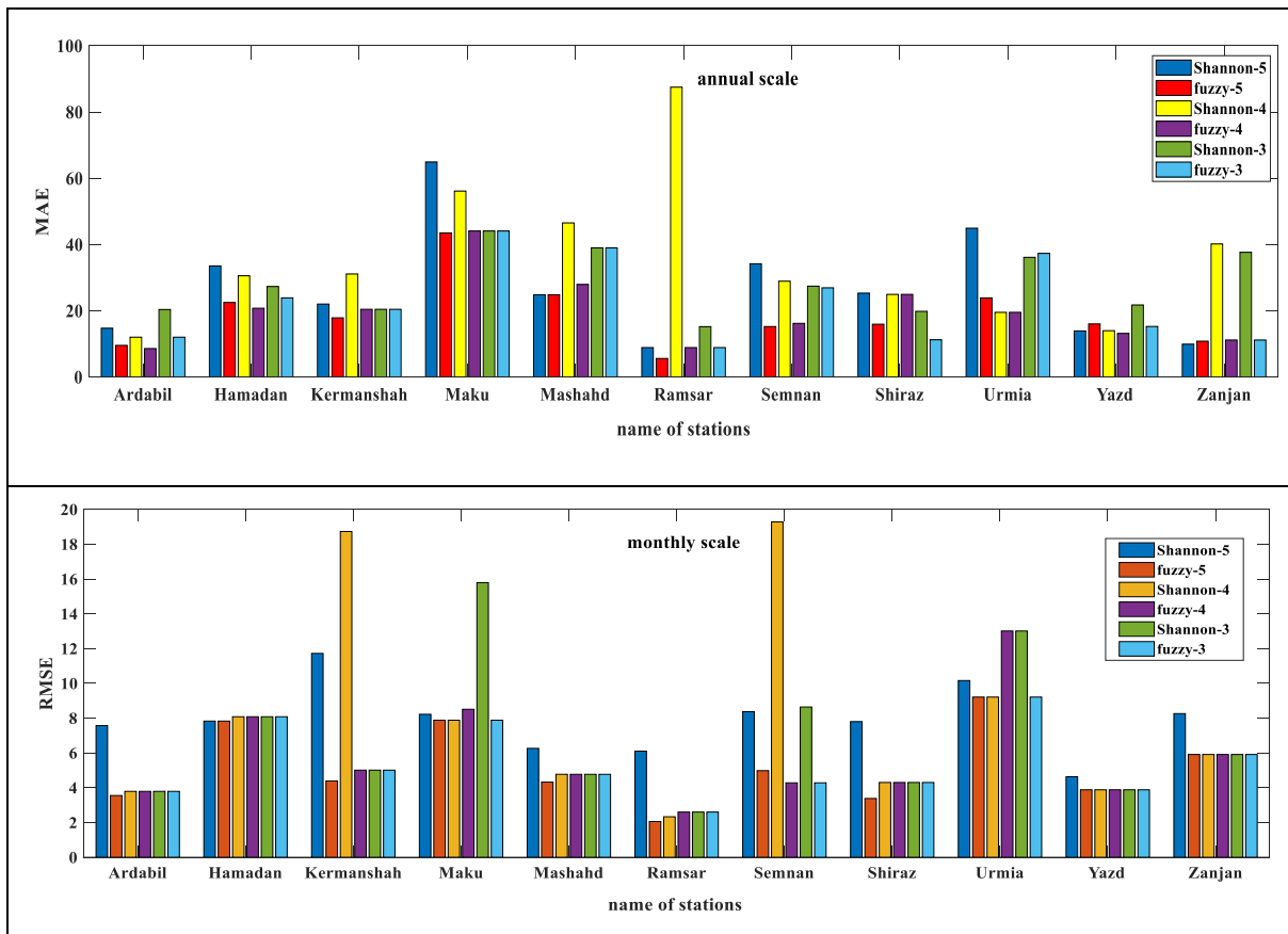
Figure 6. Comparison, the efficiency of Shannon’s entropy and fuzzy normalization methods, with a high weight of each group in all stations
