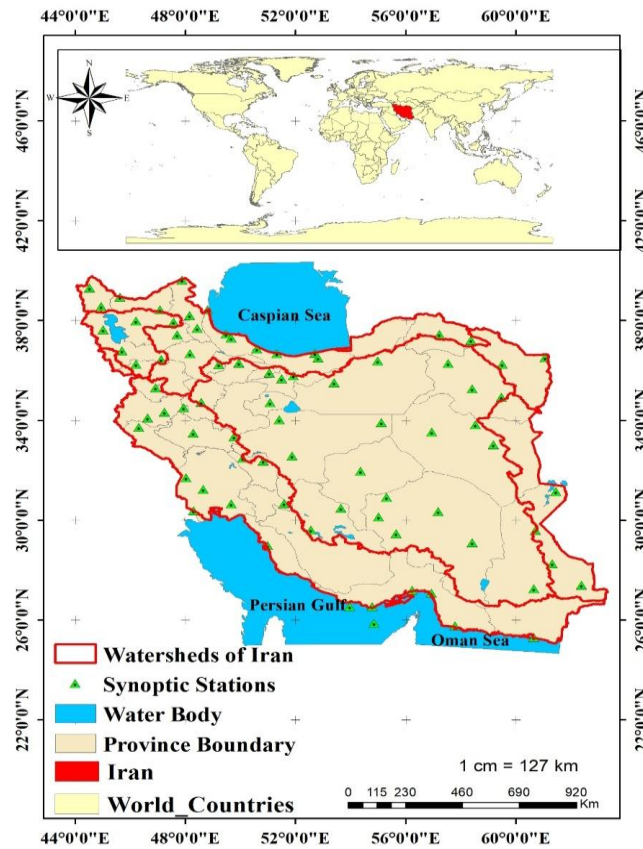
Figure 1. Location of the study area and synoptic stations in Iran
